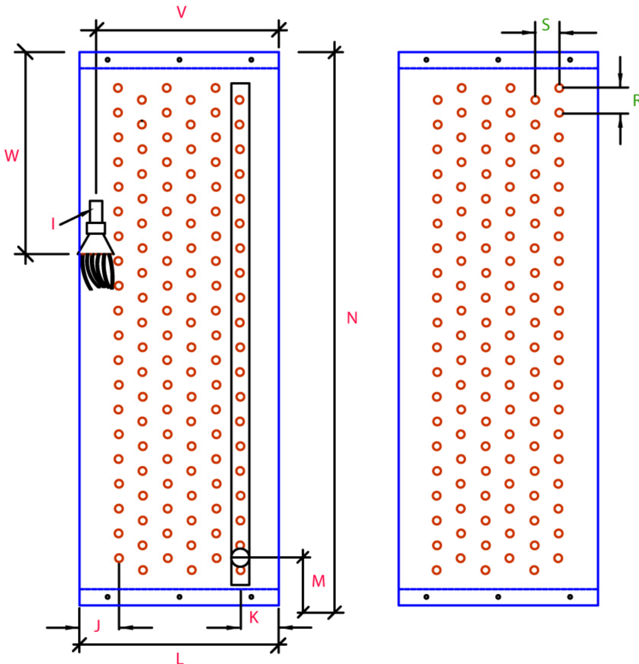
HEADER PLATE-VIEW X
