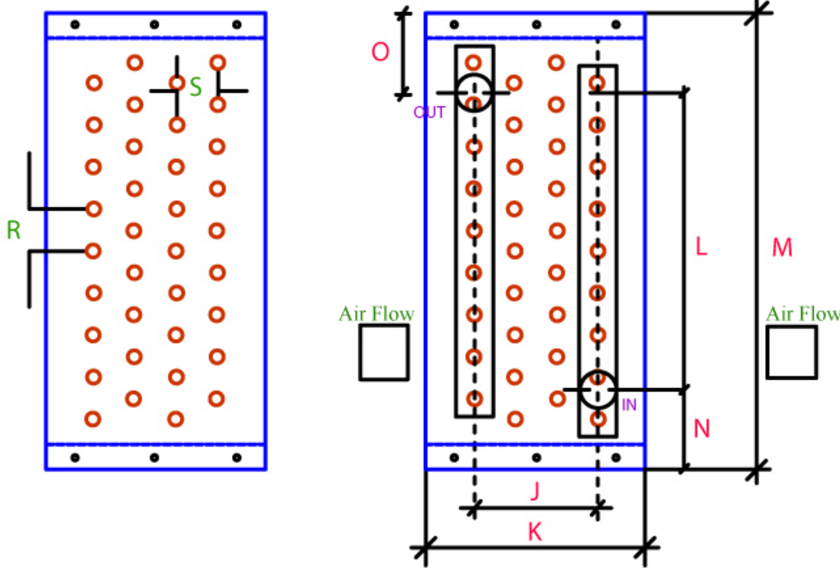
VIEW - X
